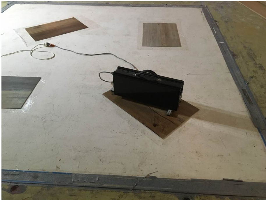
Figure 2: Tapping machine on vinyl sample on test floor
